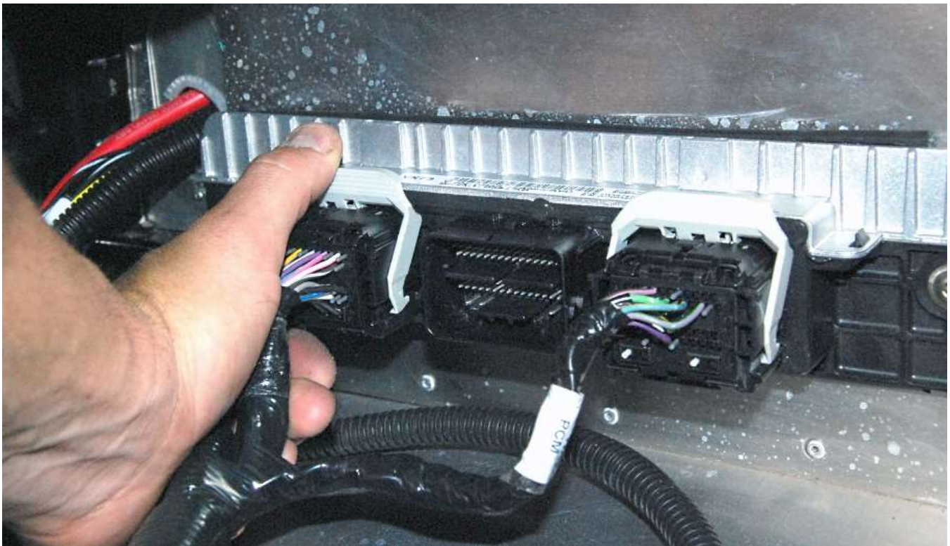
Plug the two engine harness plugs into the computer.
