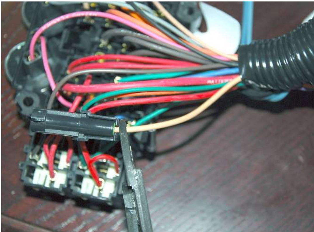
Cut the connector off the tan wire going into the harness
