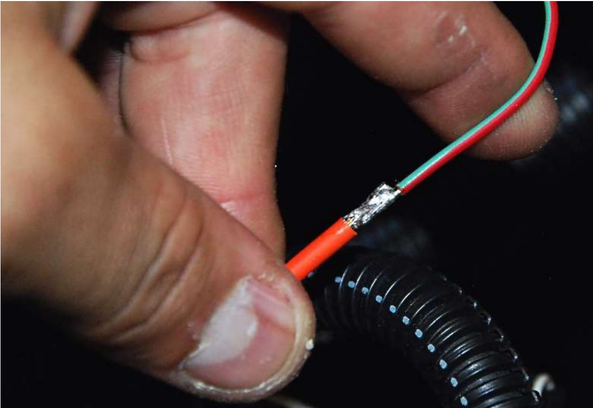
Connect the 12v start/run wire (red/green) wire to the orange coil wire.
