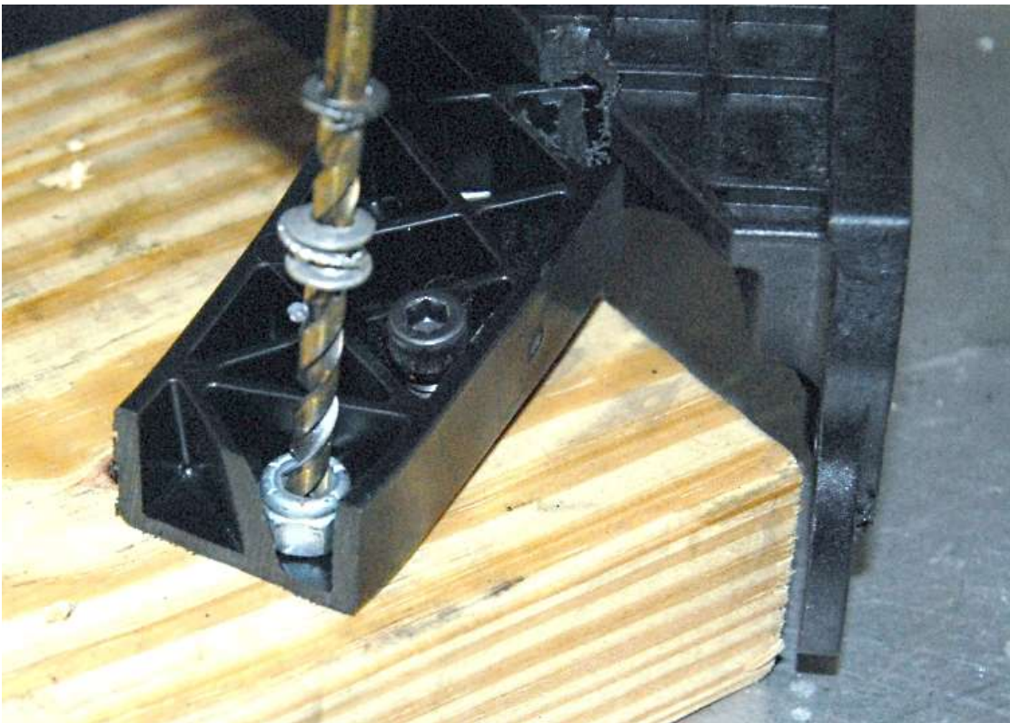
Use another lock nut and drill bit to locate the lower hole location and drill a pilot hole.
