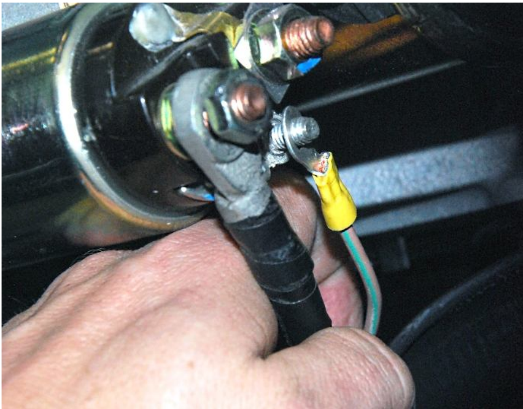
Attach the tan/green wire to the starting post on the solenoid.
