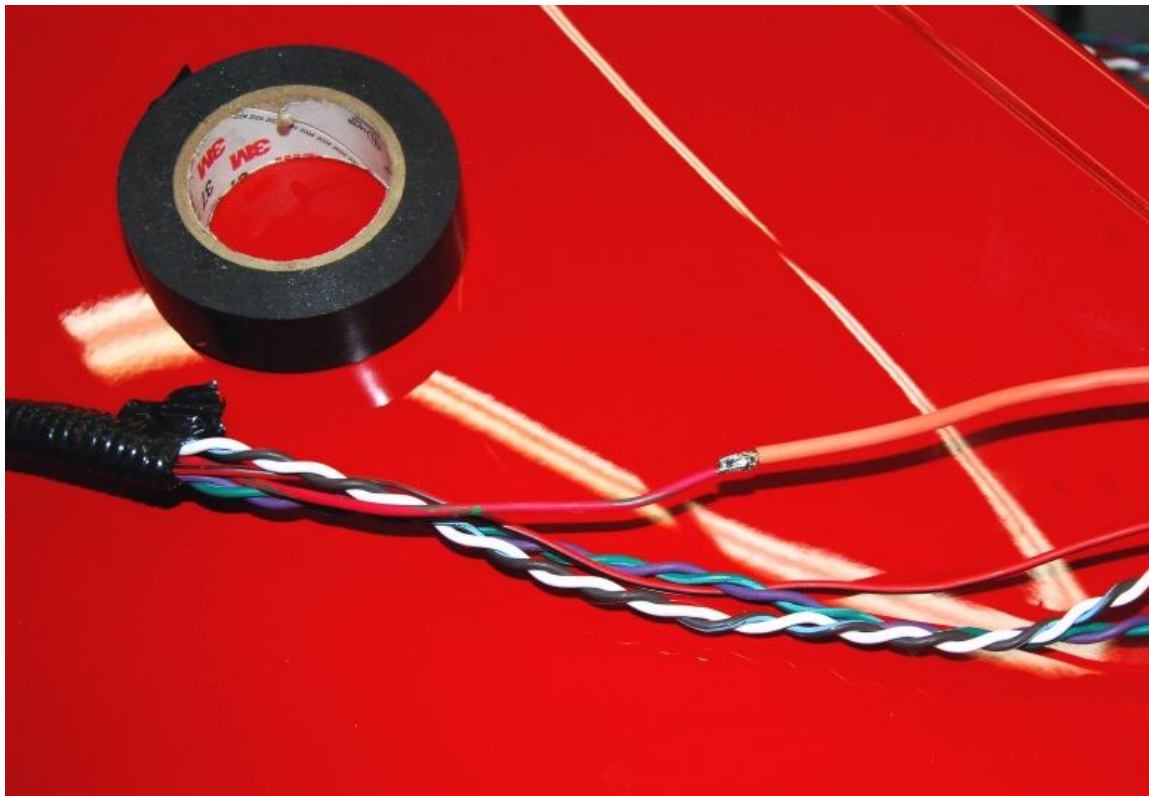
Solder the other end of the extension wire to the O 2 sensor wire.
