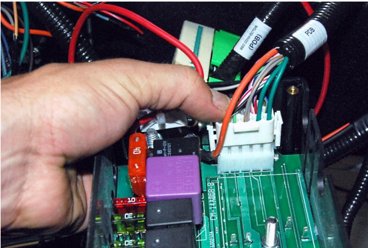
Push the white multipin connector onto the matching connector on the circuit board.
