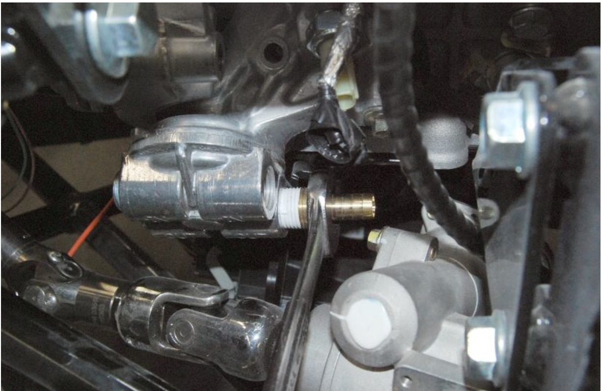
Screw the hose fittings into the rear of the spin-on adapter.
