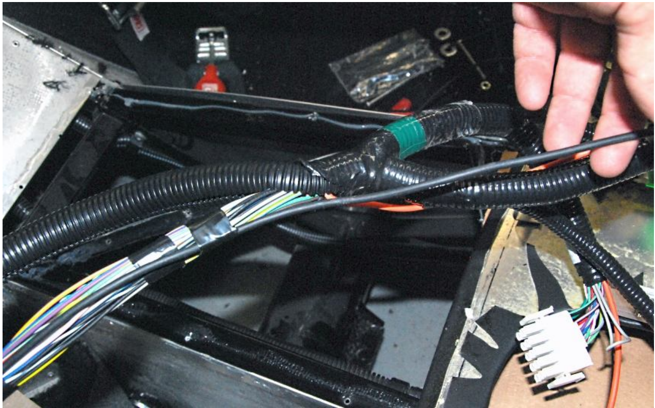
Tape the ground wire back along the harness to a common frame ground.
