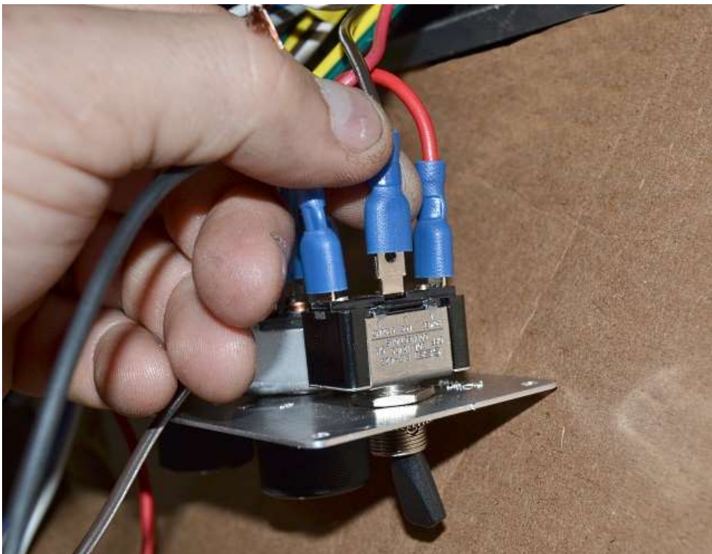
Push the brown wire onto the center of the A/C switch.
