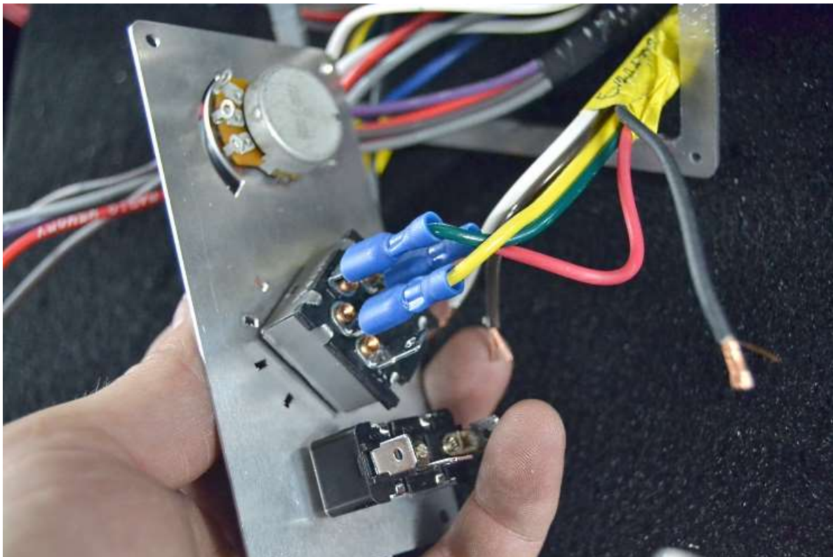
Take the “Evaporator wires and attach ¼” female connectors to the yellow, green and red wires and attach them to the rotary fan switch; Green on the top center “M” location, Yellow on the top left “L” location and the red on the top right location “H”.
