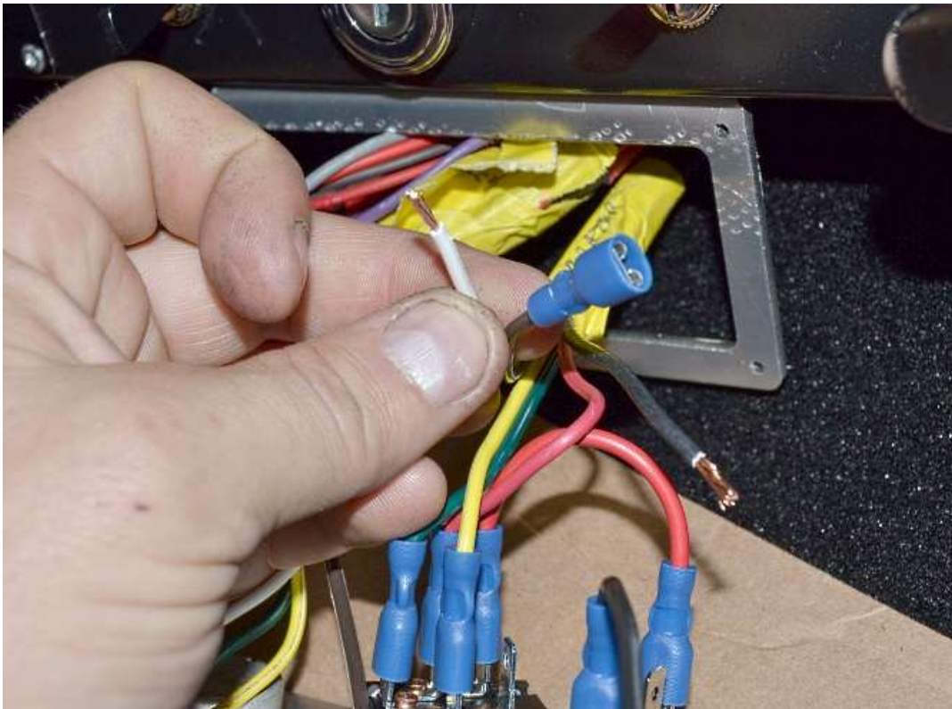
Attach a 1/4" female connector to the brown "Evaporator" wire.
